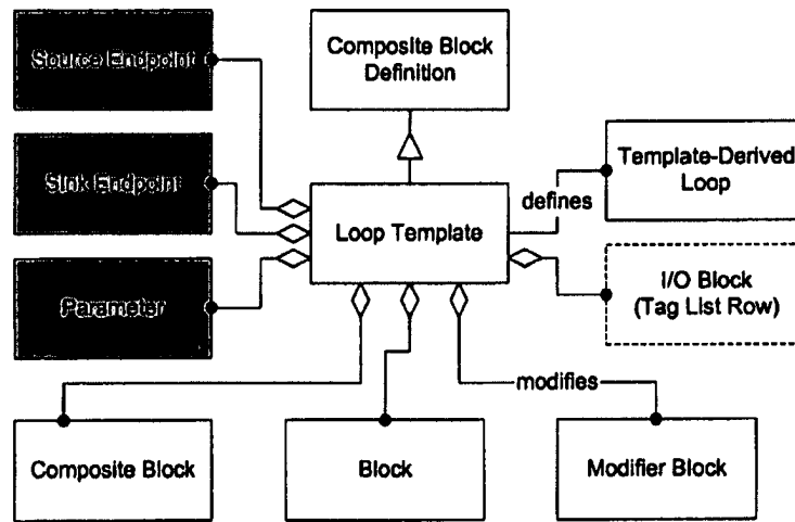
Figure 88 - Loop Template object model
